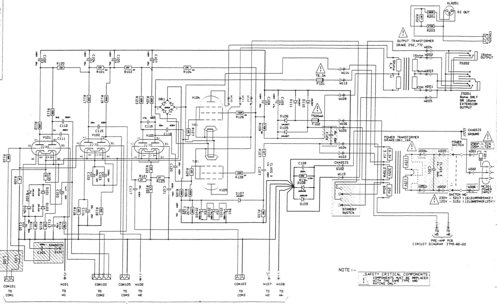
PRE-AMP PCB CIRCUIT DIAGRAM JTM3-60-02
